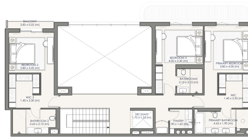
UPPER FLOOR
